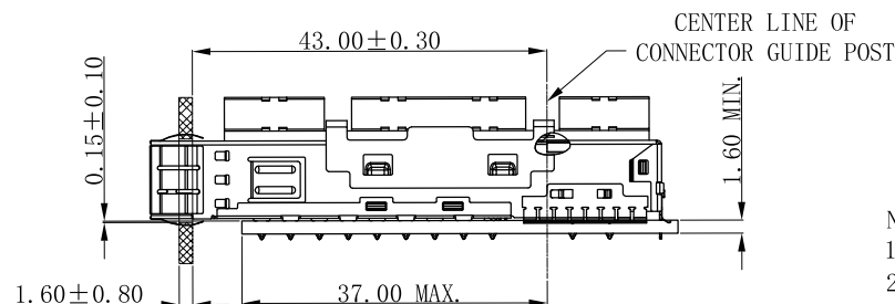
PCB LAYOUT FOR SINGLE SIDED APPLICATION
