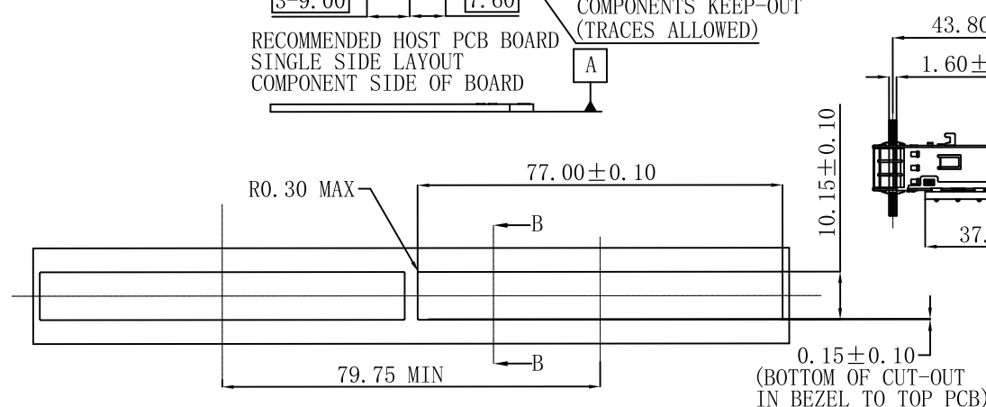
PCB LAYOUT FOR SINGLE SIDED APPLICATION
