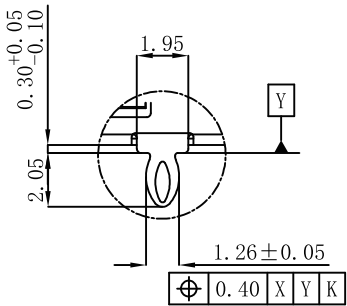
DETAIL A SCALE 5:1
