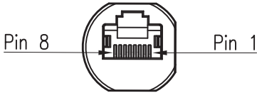
Pin Assignments Front View
