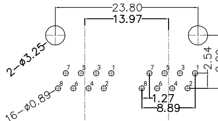
RECOMMENDED PCB LAYOUT VIEWED FROM COMPONENT SIDE
