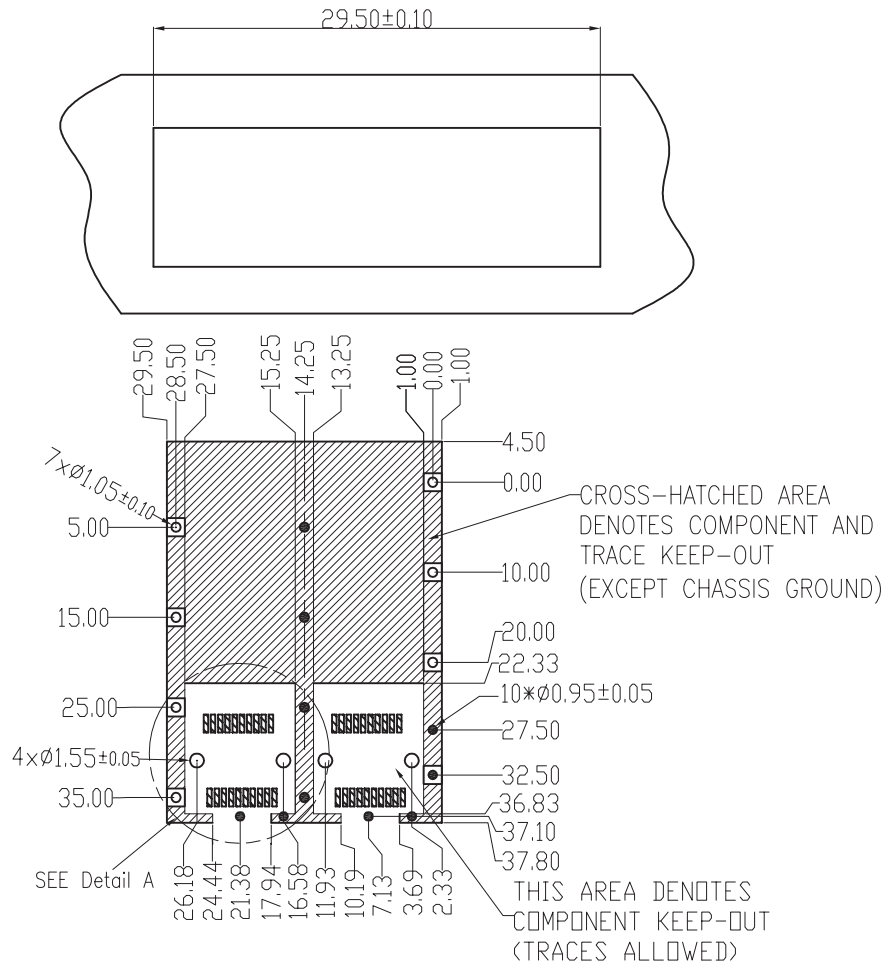
PCB LAYOUT THICKNESS=3.0MM (TOP VIEW)
