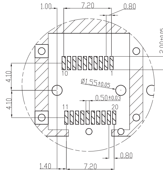
SEE Detail A SCALE 2.5:1
